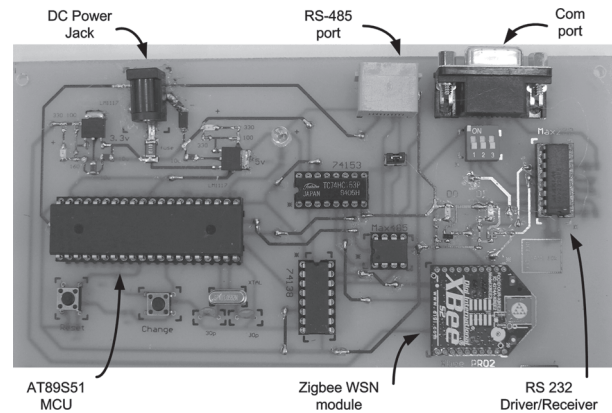
Fig. 3. The control circuit of Data Transfer Board (DTB).
