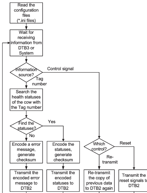
Fig. 5. The data flow of the program executed on DAS.
