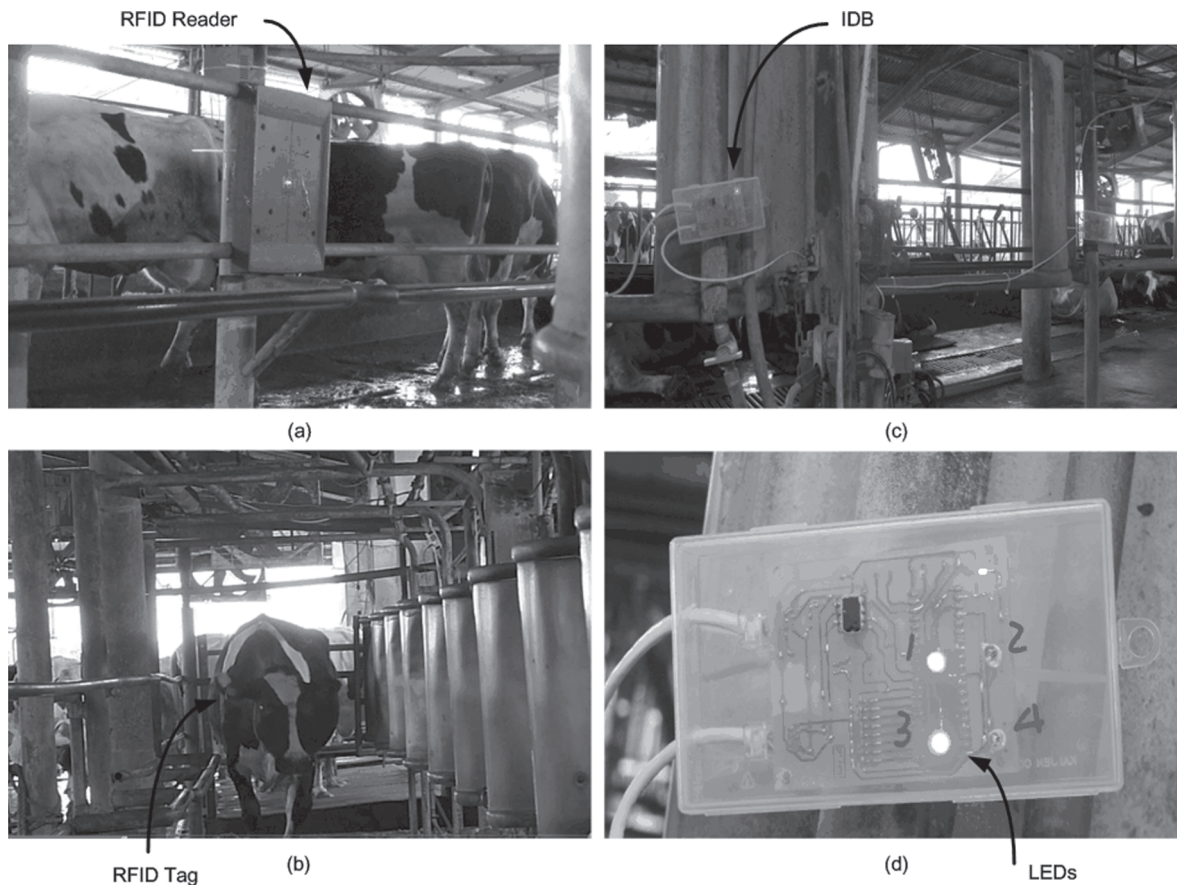
Fig. 7. (a) A RFID Reader deployed at right side of the entrance in the milking parlor; (b) A cow with a Tag passes through the entrance; (c) An IDB deployed at a fixed position in the milking section; (d) An IDB shows the health statuses of the cow.
