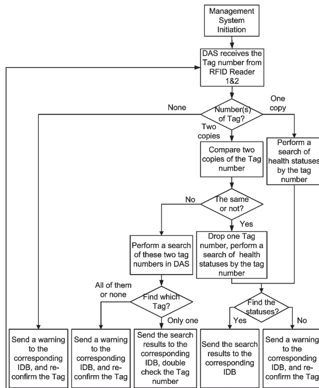
Fig. 2. The data flow of the management system.
