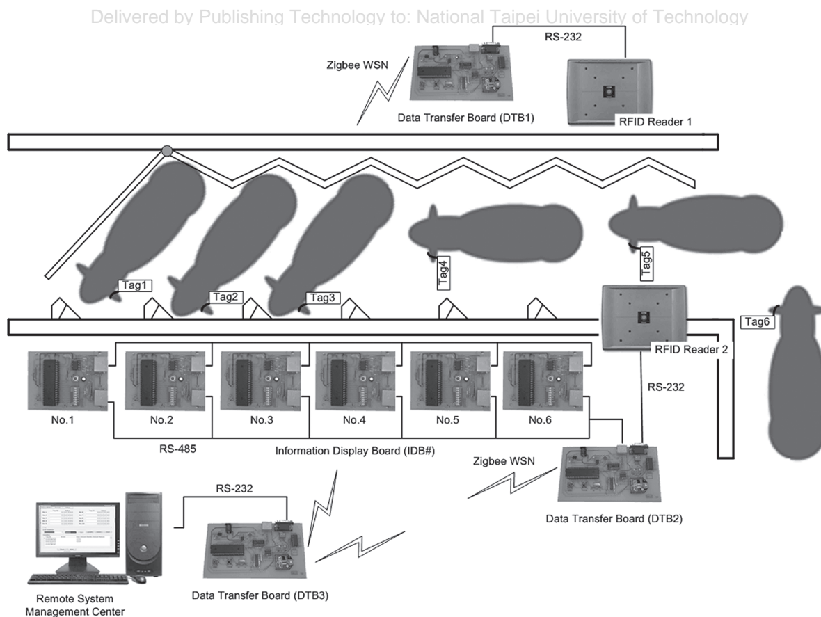
Fig. 1. The management system architecture.
